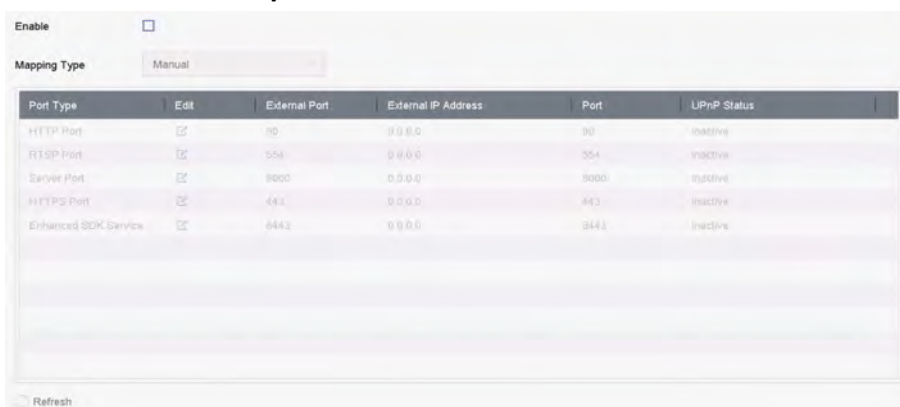
Figure 12-3 Port Mapping Setting
