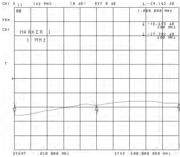
Picture 4 – input return loss, IS11, 30 kHz – 600 MHz
