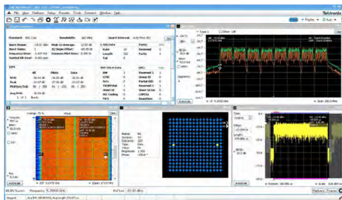
Easy analysis of WLAN 802.11ac transmitter with a WLAN preset that provides spectral emission mask, constellation diagram, and decoded burst information.
