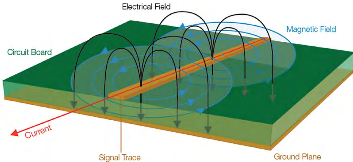
FIGURE 6. The changing voltages and currents that make up signals result in electric and magnetic fields.
