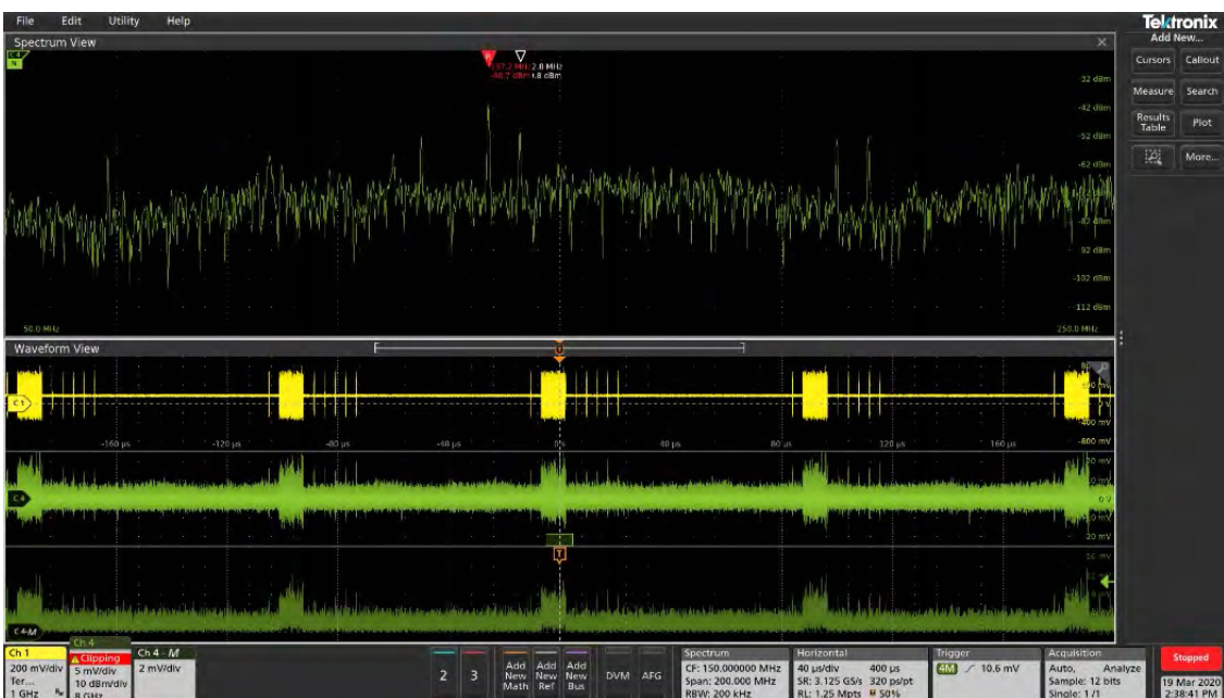
FIGURE 15. Trigger on RF Magnitude v Time on offending RF energy and observing the coincident electrical event.
