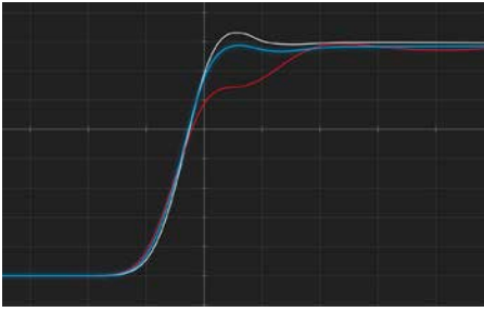
An edge loaded by Keysight N2894A probe (red) versus Tektronix TPP1000 probe (blue).
