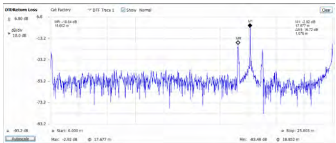
FIGURE 10. Return Loss vs. Distance.
