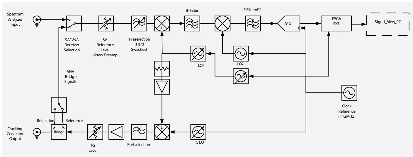
FIGURE 1. RSA500/600 Series spectrum analyzer with optional tracking generator.
