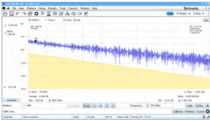
FIGURE 4. Cable Loss (Insertion Loss) vs. Frequency of 50 ft. RG-58/U coax cable with a mask applied.
