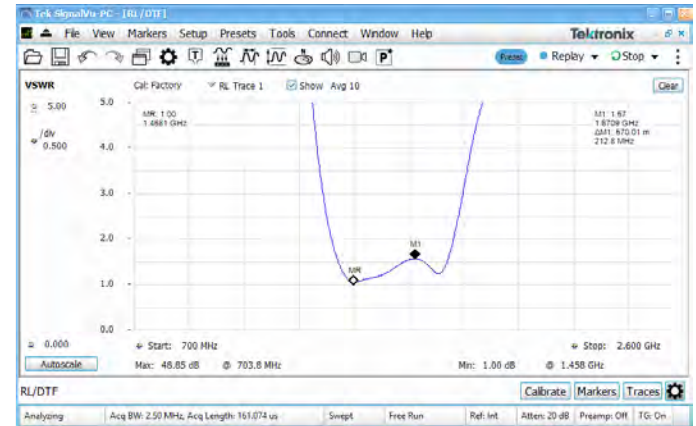
FIGURE 3. VSWR vs. Frequency of a bandpass filter.
