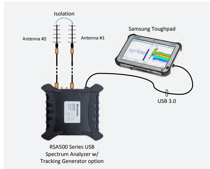
FIGURE 13. Co-Located Antenna Isolation Test Setup.
