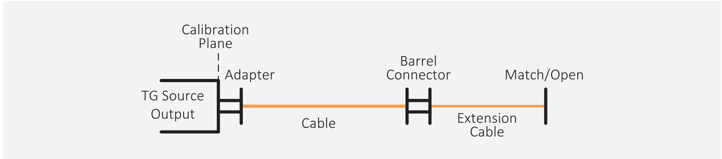
FIGURE 9. Typical Distance to Fault Measurement Setup.
