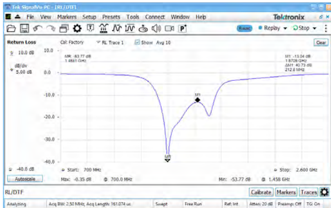
FIGURE 2. Return loss vs. Frequency of a bandpass filter.
