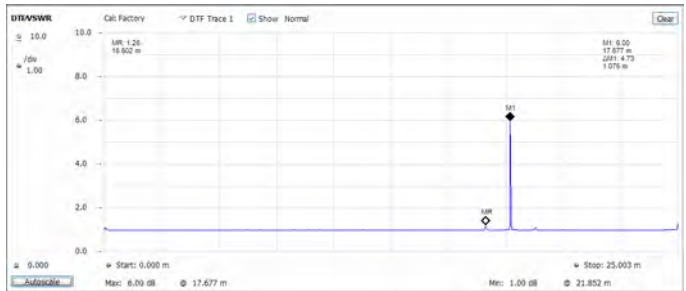
FIGURE 11. VSWR vs. Distance.
