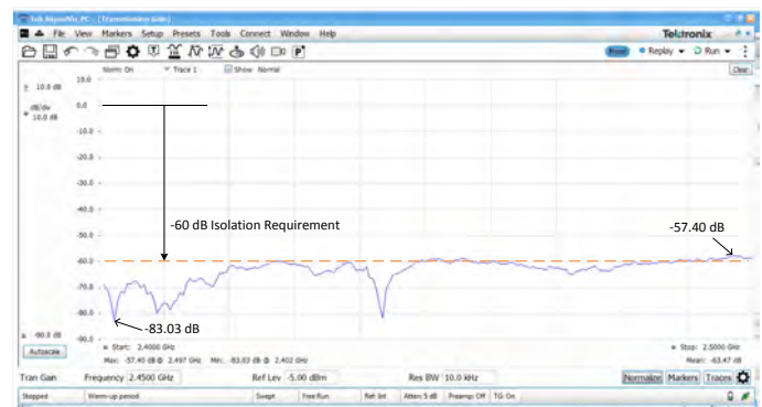
FIGURE 14. Isolation vs. Frequency Measurement
