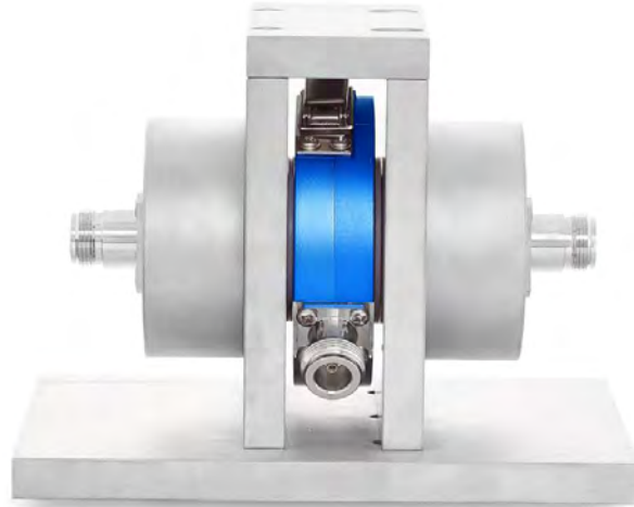
Picture 2: TBCP2-CAL RF current probe calibration fixture
