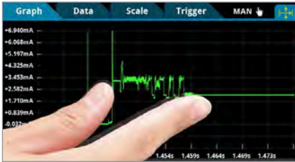
Capture the current drain from all the operating states – sleep mode to active transmit mode – of a component or a product with the DMM7510's digitizing function. Focus in on characteristics of the wave shapes with the touchscreen pinch and zoom features.
