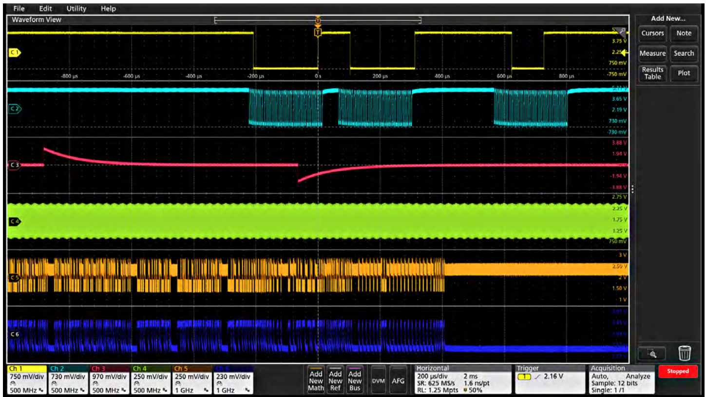
Using multiple channels to visualize multiple clock and data lines.
