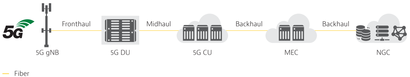
Figure 2 : Typical 5G Network Architecture
