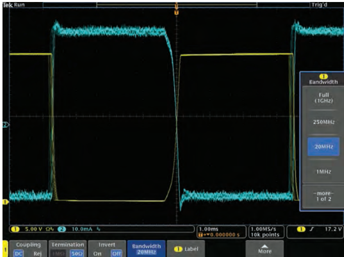
Figure 10. Bandwidth Limiting Filters Available on an MDO4000 Series Oscilloscope with a TDP1000 Attached.
