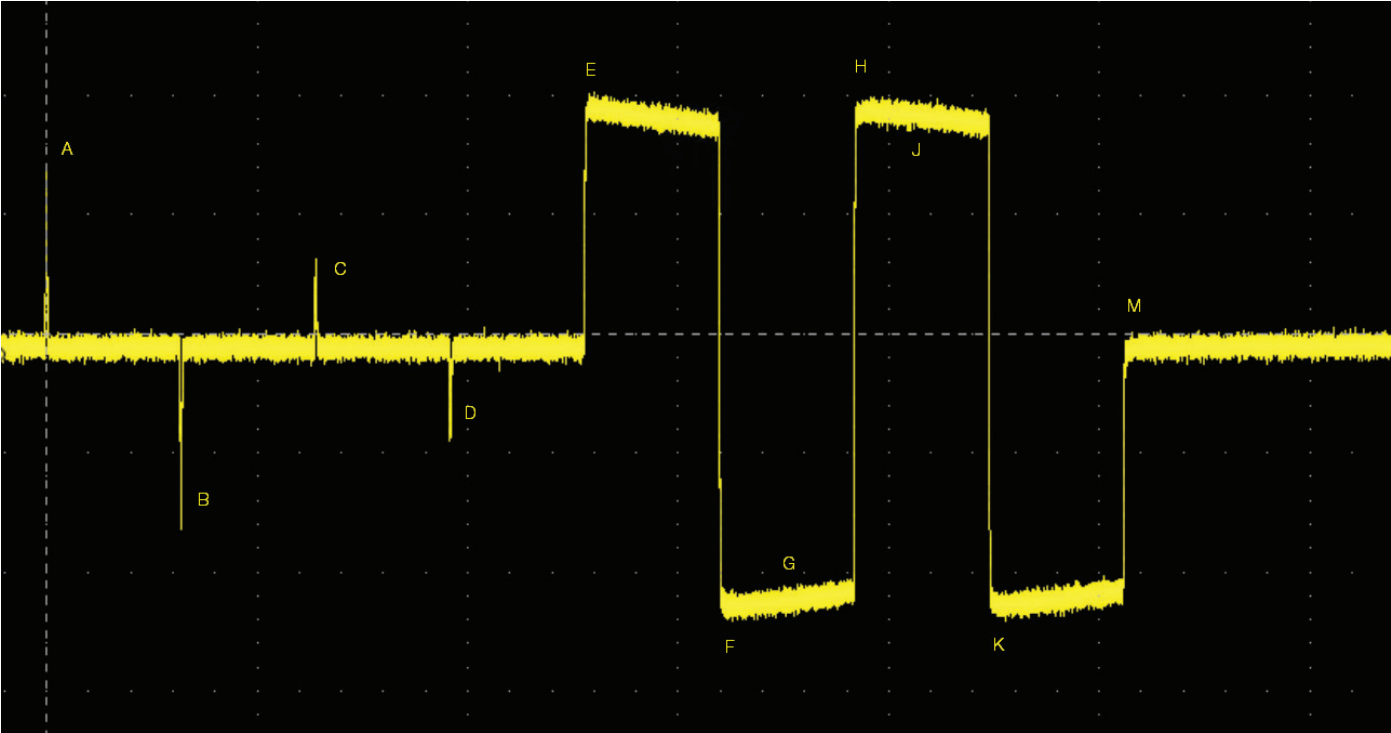
Figure 2. Single cycle of 1000BASE-T Test Mode 1 signal.
