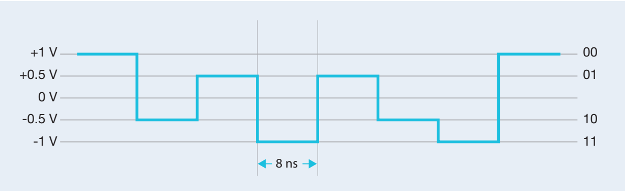
Figure 1. 1000BASE-T Multi-level PAM5 encoded signal.
