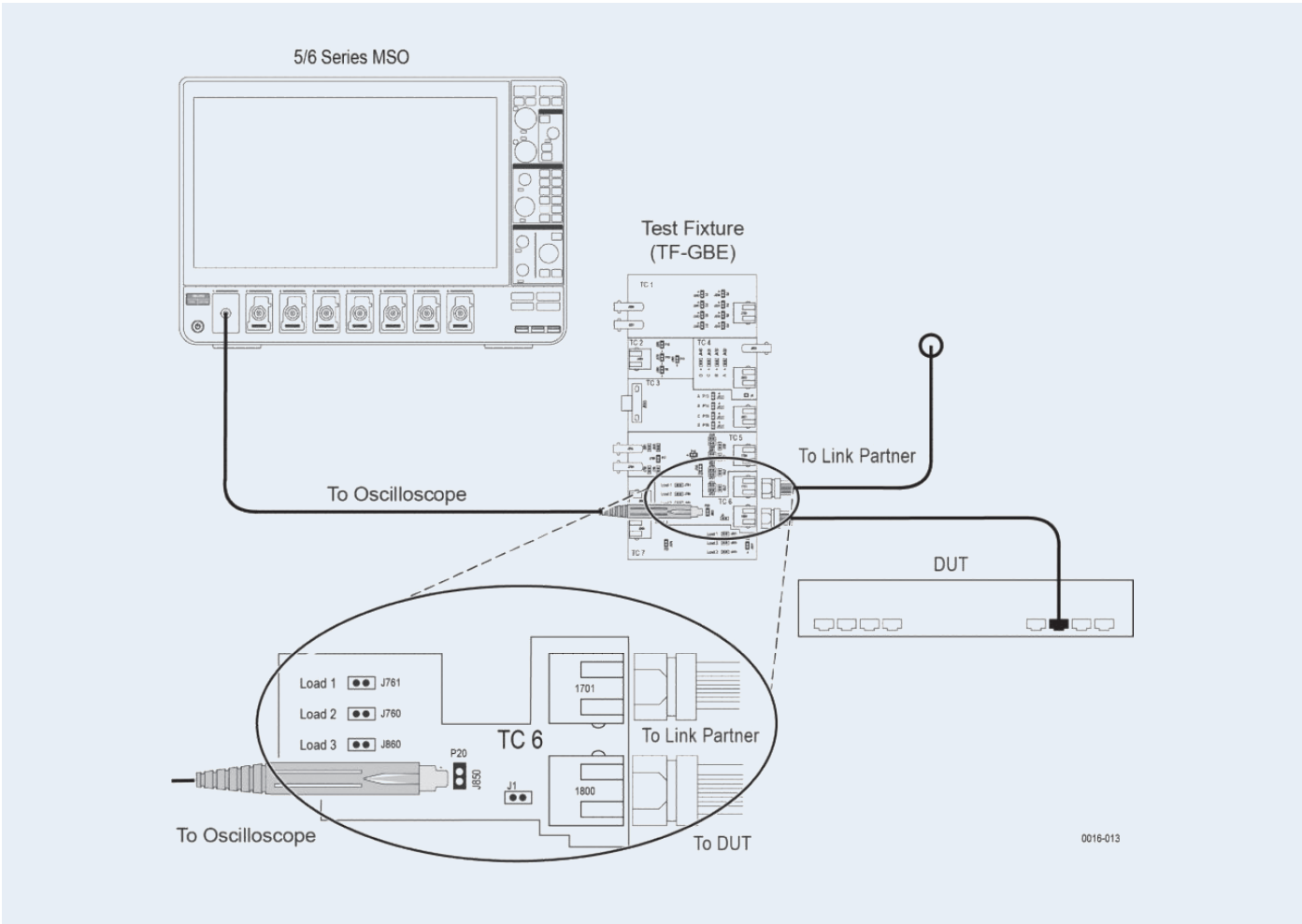
Figure 12: Test setup with a link partner
