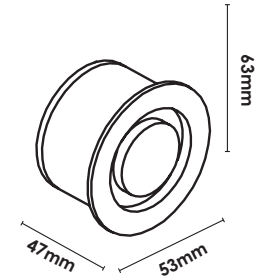
CUTOUT WITHOUT CANISTER Ø54MM
