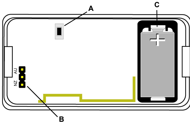
Figure 1 EN1224/EN1224-ON components
