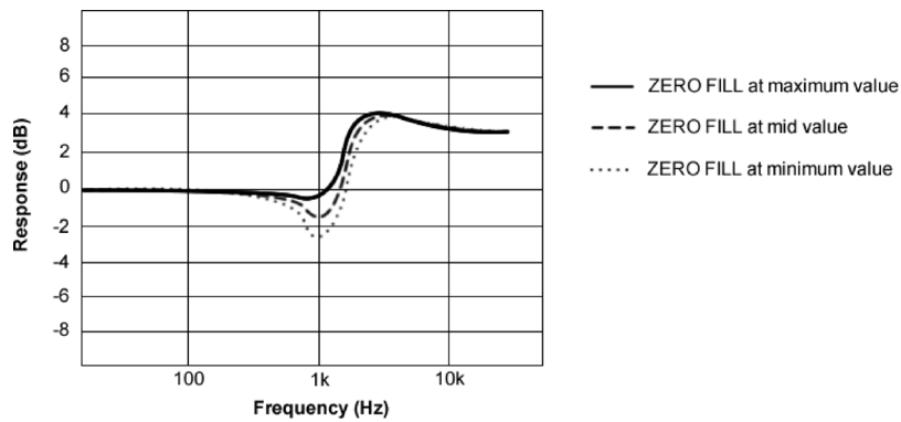
Figure 155: Frequency response for different ZERO FILL values
