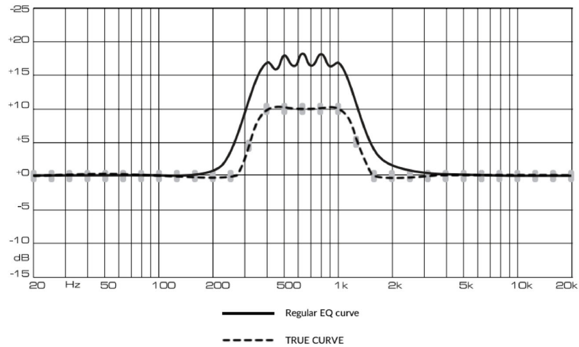
Figure 82: TRUE CURVE
