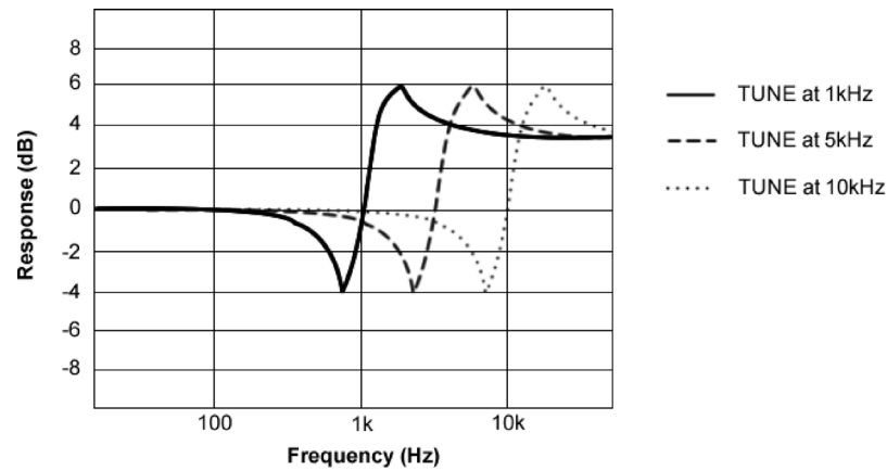
Figure 153: Frequency response for different TUNE values
