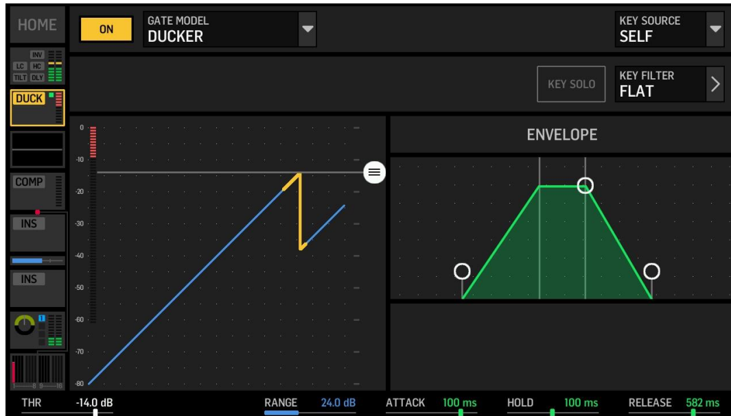
Figure 117: Ducker
