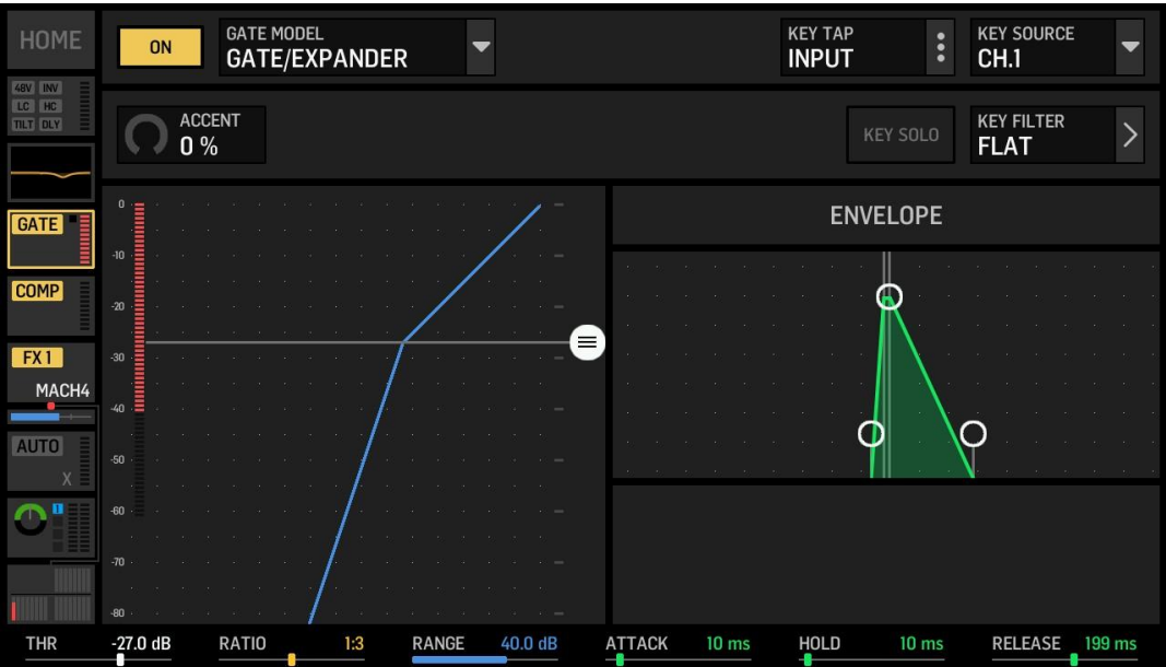
Figure 94: WING Gate/Expander
