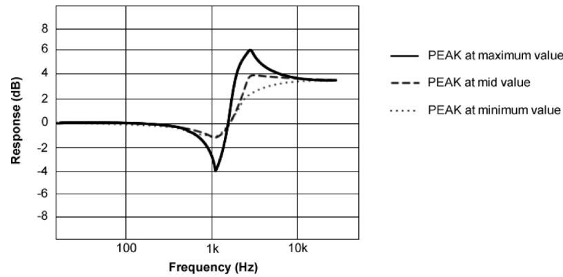
Figure 154: Frequency response for different PEAK values
