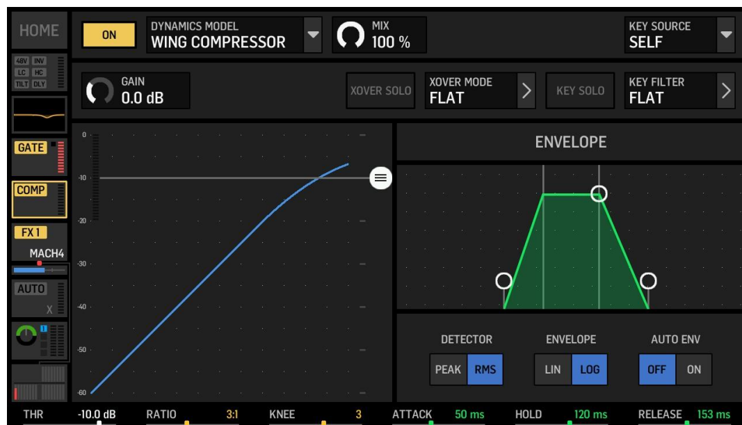
Figure 92: WING Compressor
