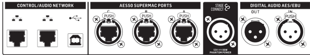
Figure 6: ETHERNET/AES50/Control/StageConnect connectors
