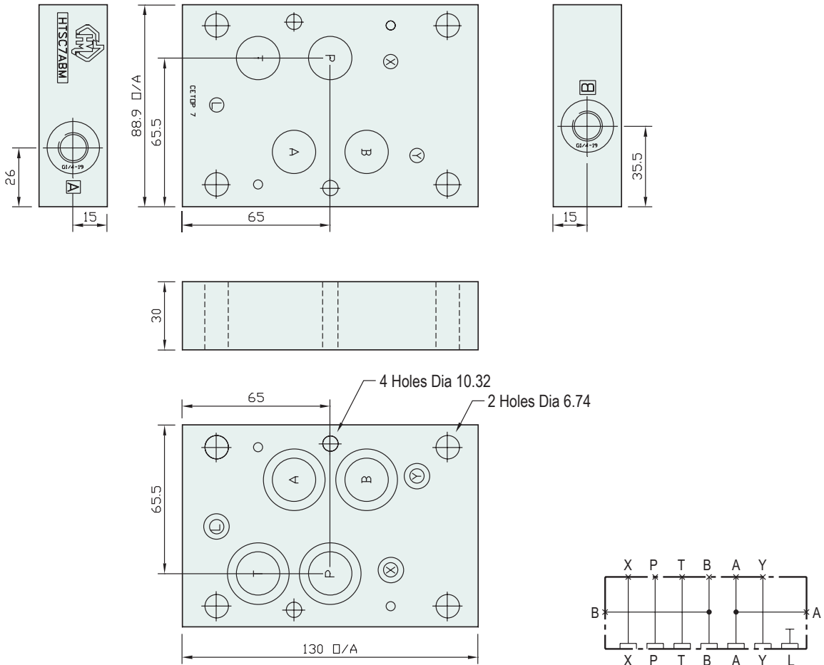
Manifold Circuit
