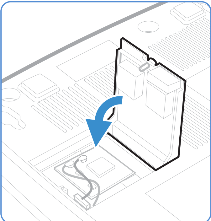
PC42E-T - Adhere antenna
