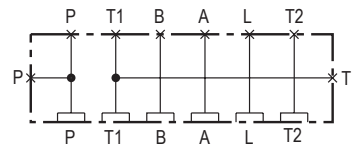
Manifold Circuit
