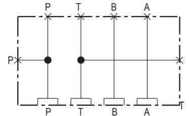
Manifold Circuit
