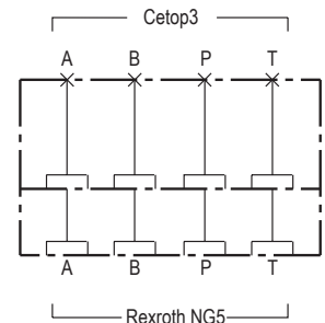
Manifold Circuit
