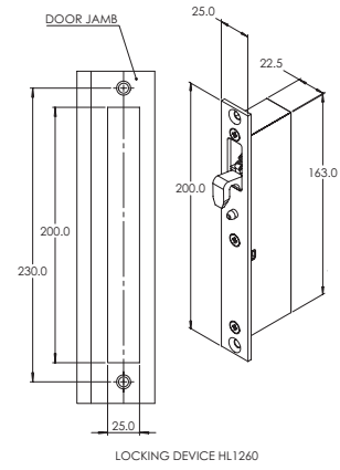
Locking Device HL1260
