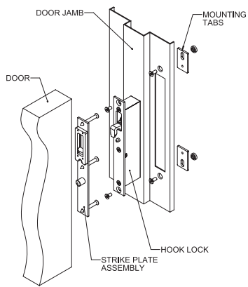
HL1260 Hook Lock Mortise Mount
