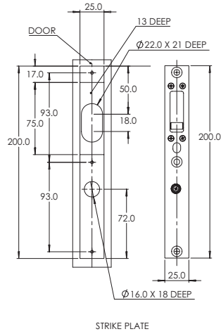
Strike Plate HL1260
