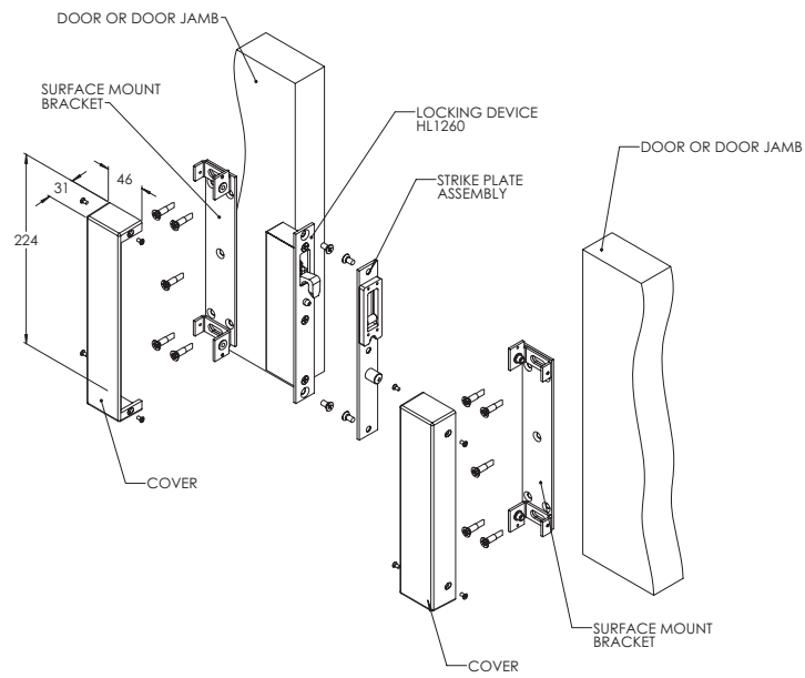
HL1260 Surface Mount Box
