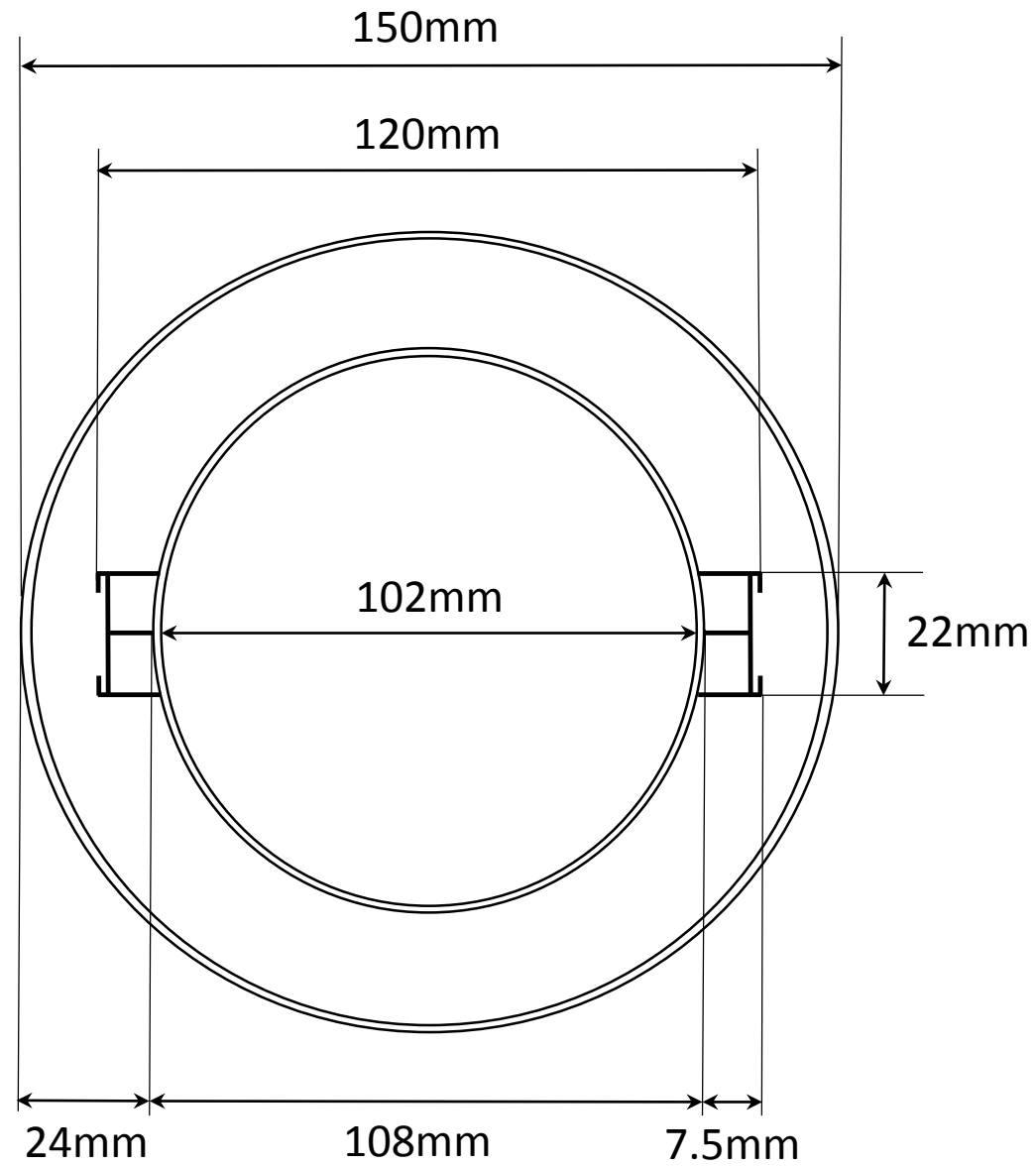
AH-06MB - HL Implant Frame for AH0621 & NQ12 Smoke
