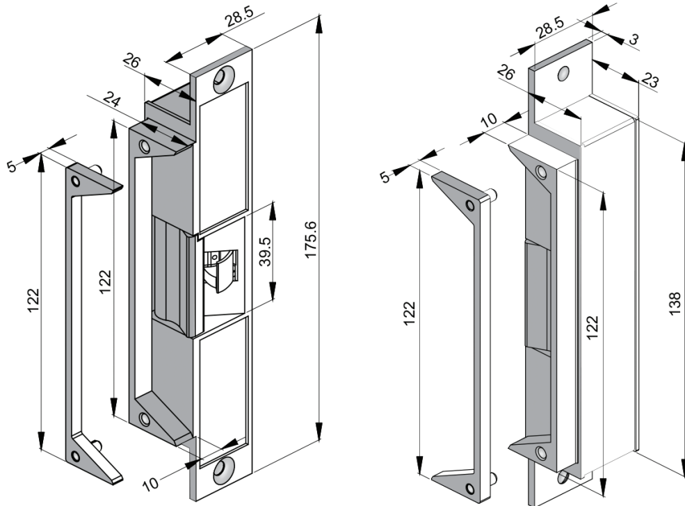
Dimensions (mm)
