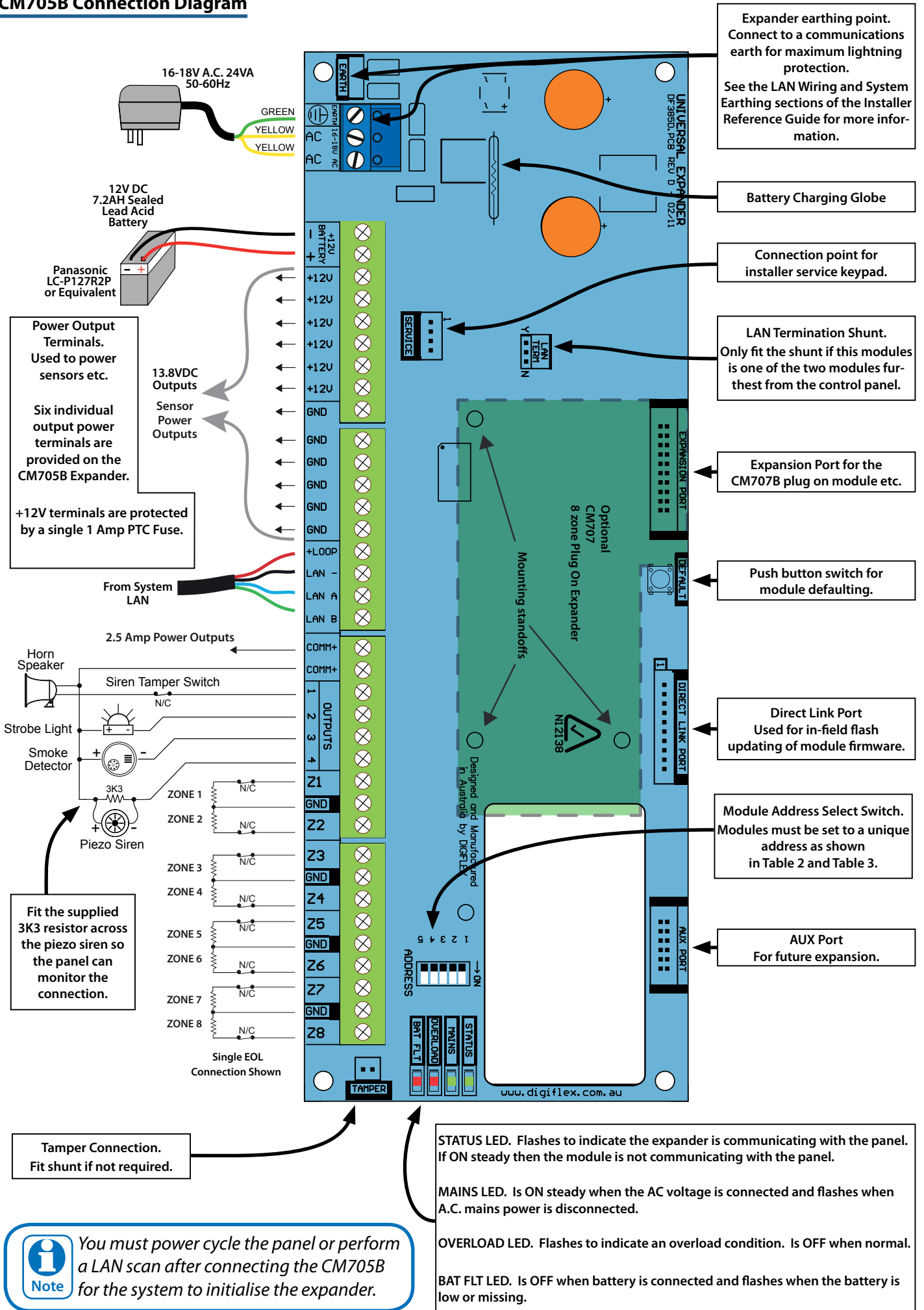
Figure 5: Connection Diagram
