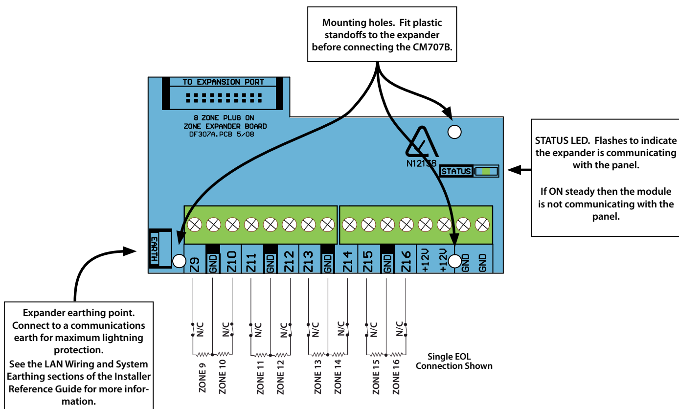
Figure 6: CM707B Plug On Zone Expander
