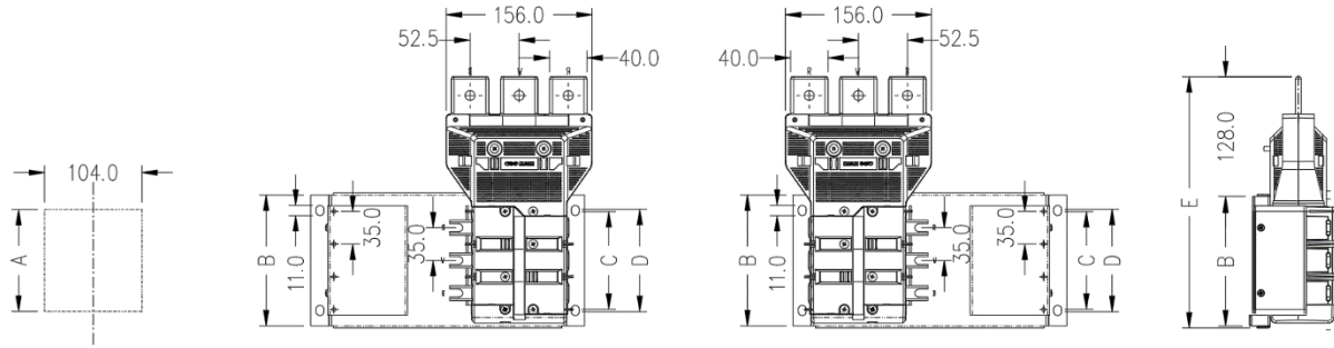
ESCUTCHEON CUTOUTS
