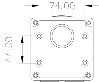
MOUNTING HOLE DETAIL
