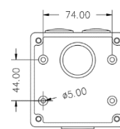
MOUNTING HOLE DETAIL
