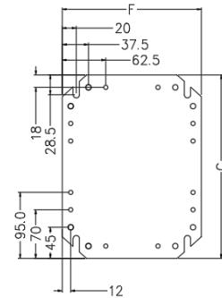
GEAR TRAY
