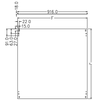
GEAR TRAY
