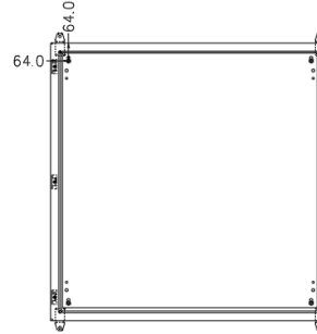
FRONT ELEVATION FRONT DOOR REMOVED
