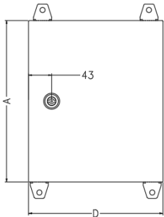
FRONT ELEVATION
