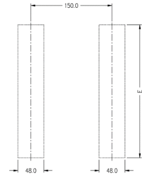
ESCUTCHEON CUTOUTS
