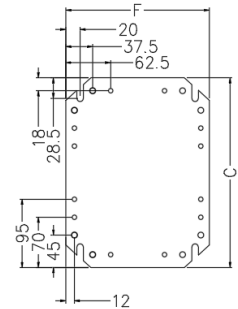
GEAR TRAY
