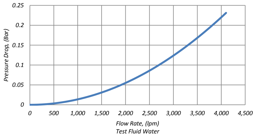
Performance Curve - 164mm Coupling
