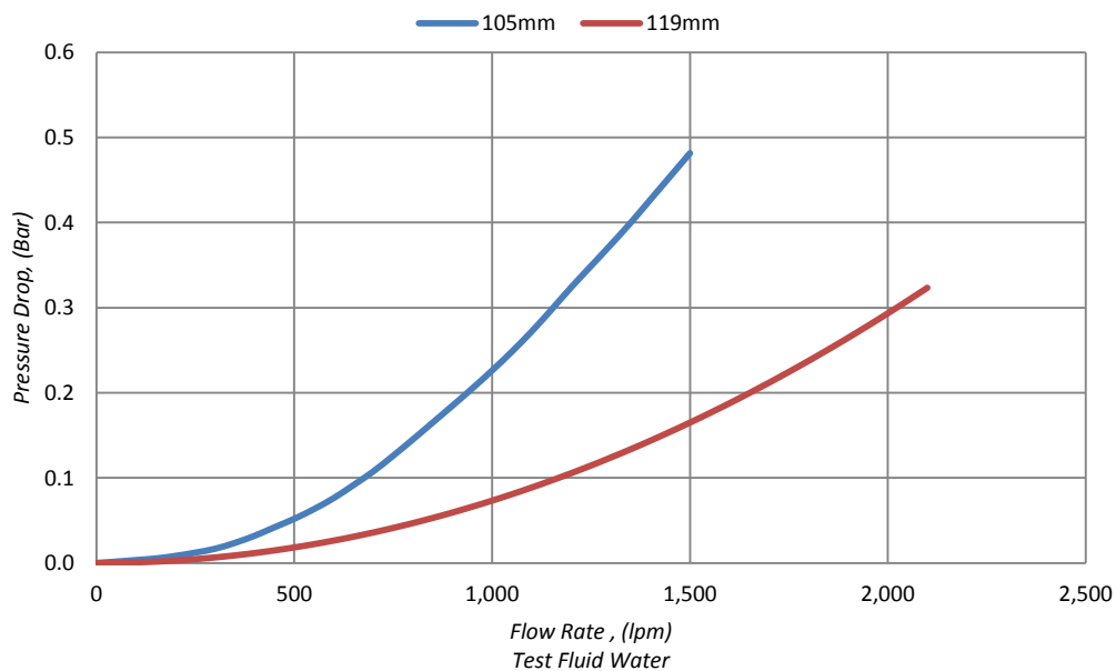
Performance Curves -105mm & 119mm Couplings
