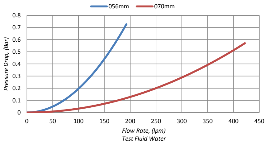
Performance Curves 056mm & 070mm Couplings
