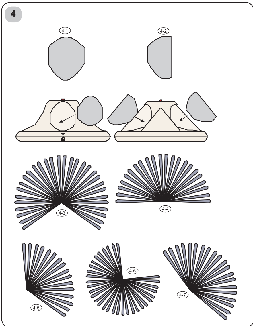
DS9370/DS9371 TriTech Ceiling Mount Passive Infrared Detector/Microwave Intrusion Detector Installation Instructions
