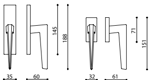
C218S - fixed window slider
