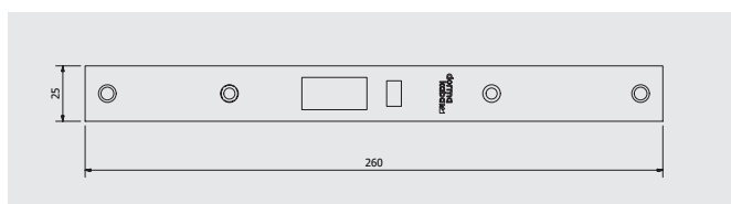
SB260 Extended Face Plate
