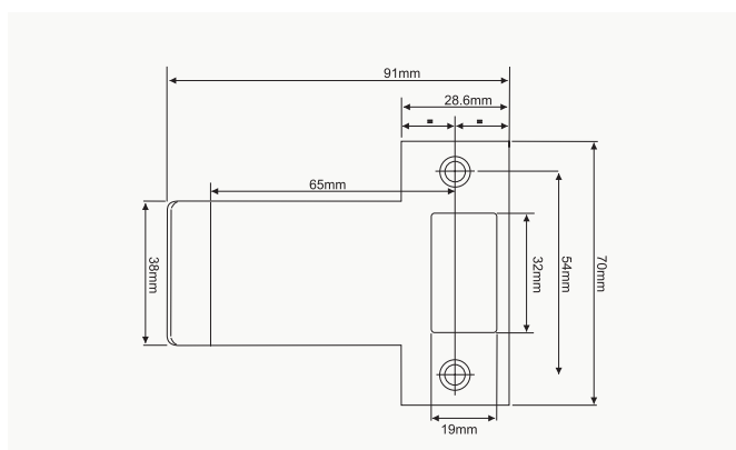
MS205 Extended Strike 65mm
