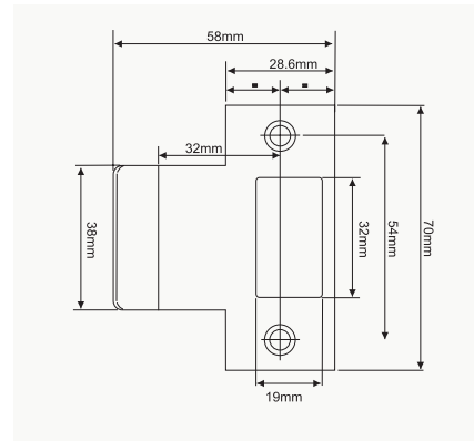
MS201 Extended Strike 32mm
