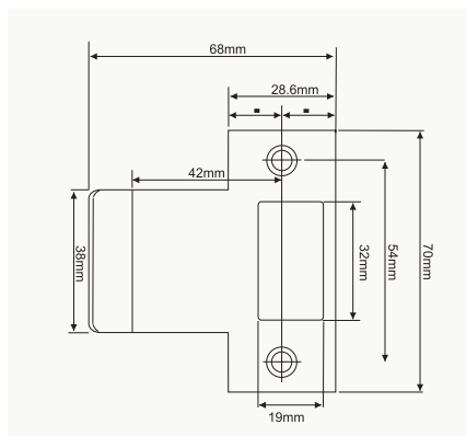
MS203 Extended Strike 42mm
