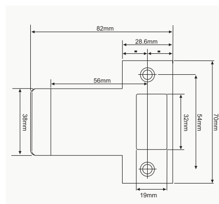
MS204 Extended Strike 56mm
