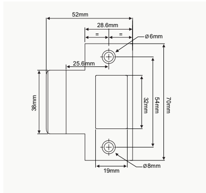
MS207 Extended Strike 25.6mm
