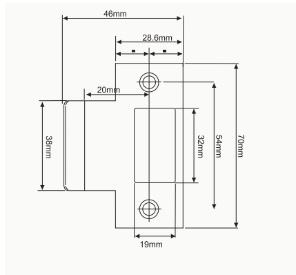
MS200 Standard Strike 20mm
