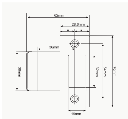
MS202 Extended Strike 36mm
