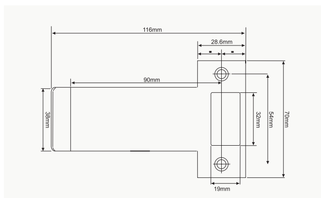
MS206 Extended Strike 90mm
