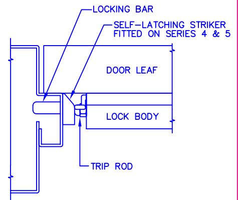
LOCKED POSITION
