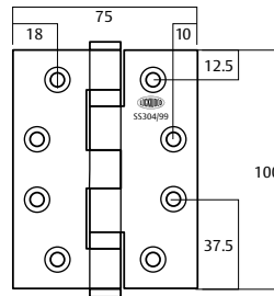
Overall dimensions
