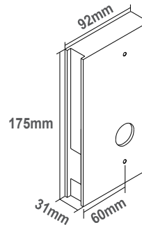
LB18 TO SUIT LOCKWOOD 3782 / KABA SBM2 WITH CYLINDER & SPINDLE HOLE
