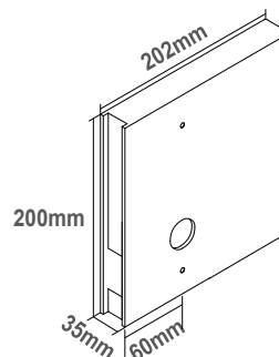
LB18P TO SUIT LEGGE 995mf WITH CYLINDER & SPINDLE HOLE
