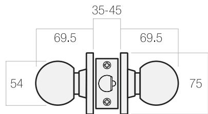
Dimensions (mm)
