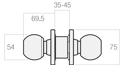
Dimensions (mm)
