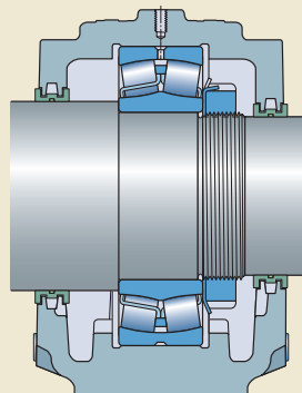
Stepped shaft with bearing on a cylindrical seat
