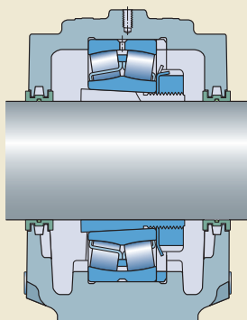
Plain shaft with bearing on an adapter sleeve
