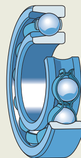
Bearing with filling slots
