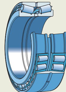
TDO design
