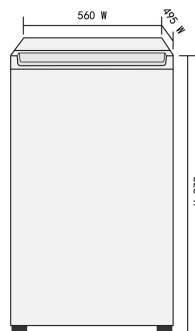
HRZ130: Height: 828mm/Width: 560mm/Depth: 495mm
