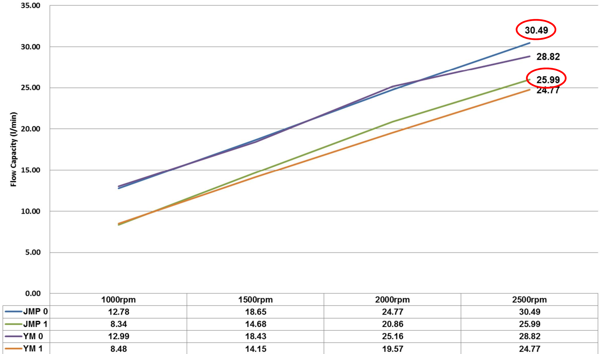
JMP YM08IH VS YANMAR 128397-42500 (JP 10-24509-01)
