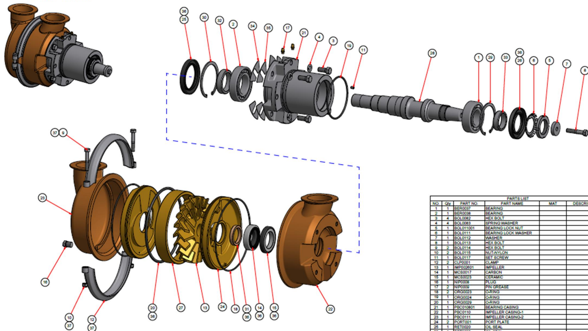
PUMP ASSY - PUA006401
