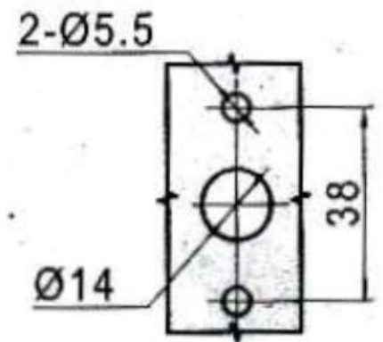
Panel Drilling
