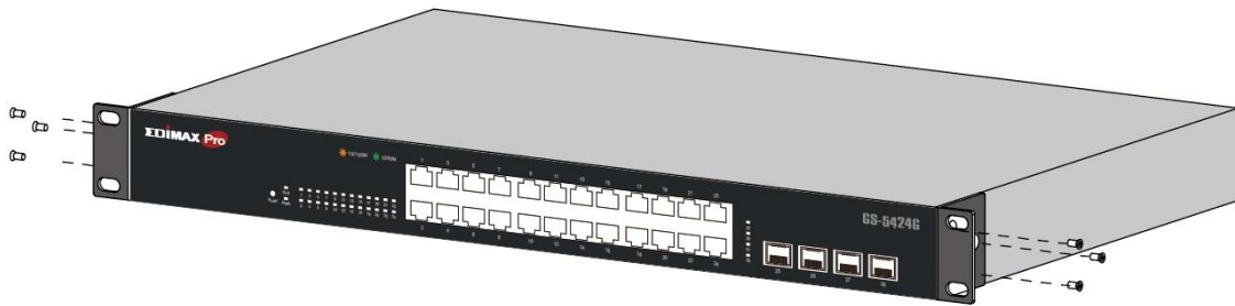
Figure 5 - Bracket Installation
