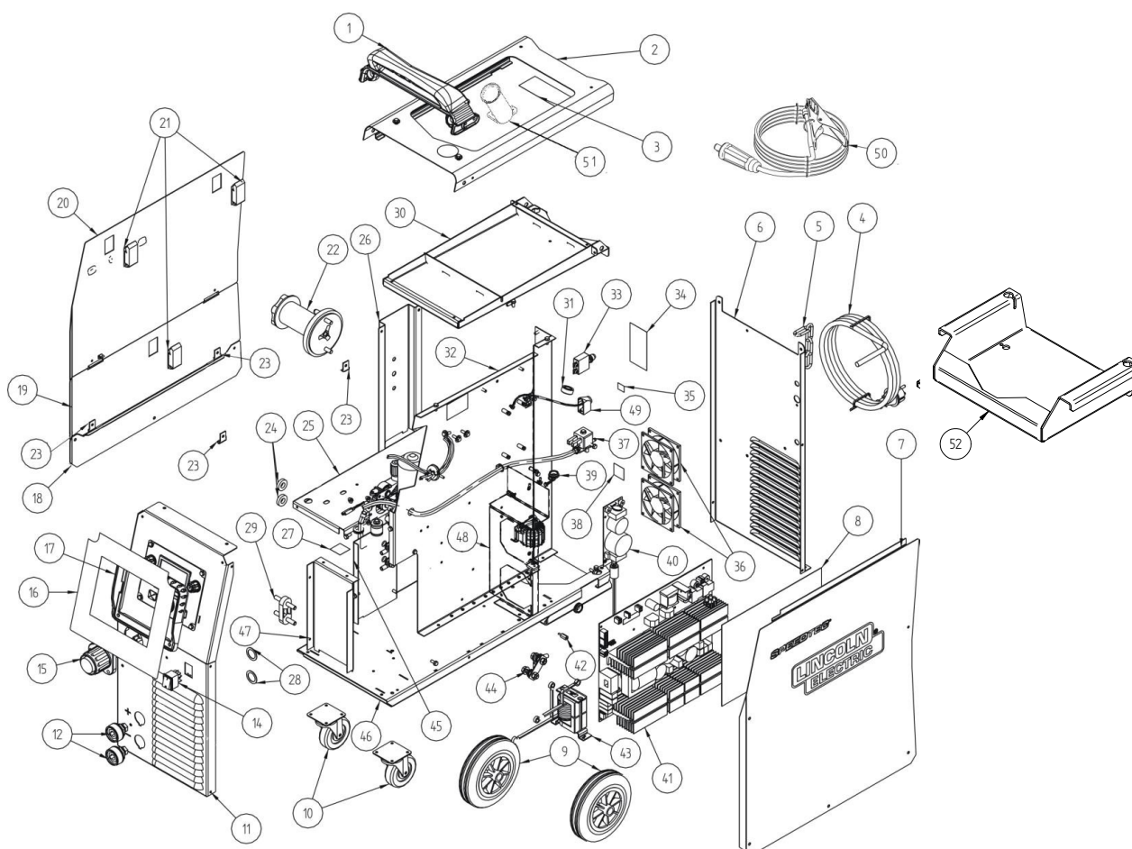
Figure A: SPEEDTEC 215C Machine Central Assembly
