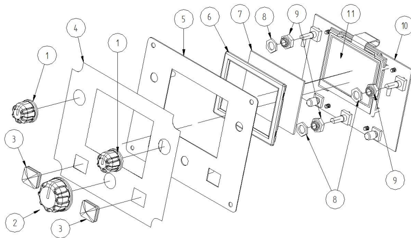
Figure B: SPEEDTEC 215C Machine Front Assembly
